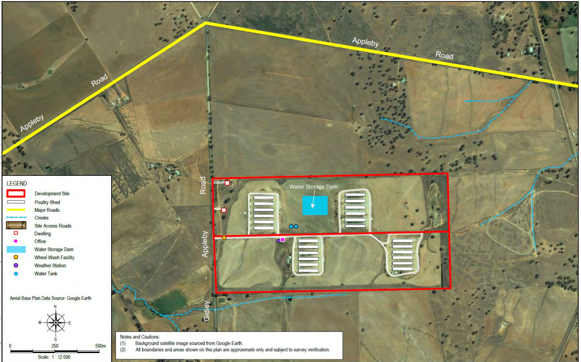
Gidley Poultry Production Complex Onsite Water Bodies FIGURE 2
