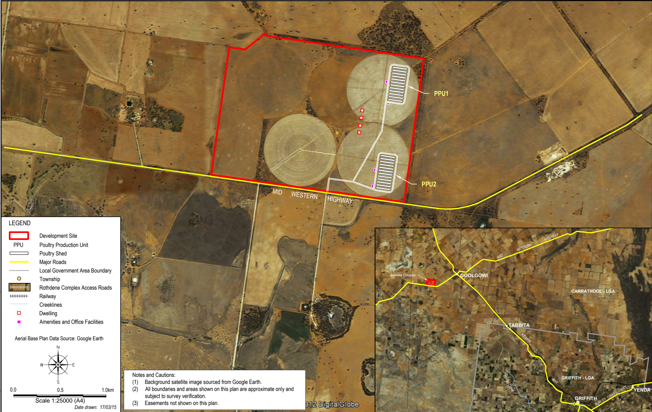
Jeanella Poultry Production Complex Location Plan FIGURE 1
